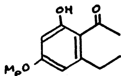
O-Methylcurvulinic acid
