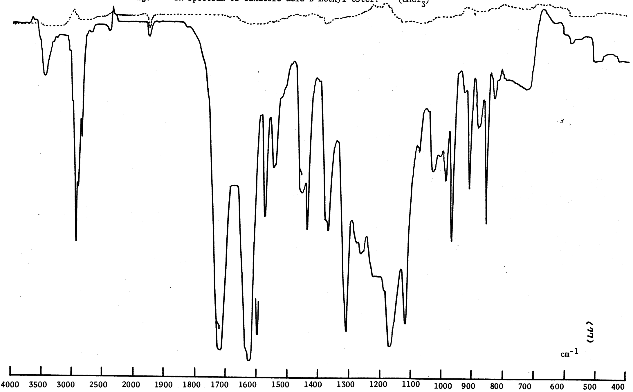
Fig. IR spectrum of lunatoic acid B methyl ester. (CHCl 3 )
