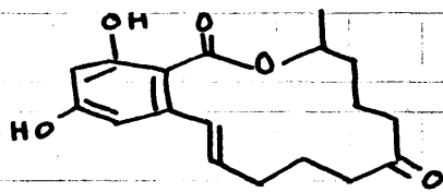
zearalenon (ref. (44))
