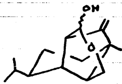
prehelminthosporol
