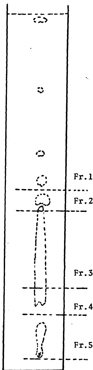
Fig. 2-2 TLC of the EtOAc-soluble strongly acidic fraction of the culture filtrate of Cochliobolus lunata IFO 5997
