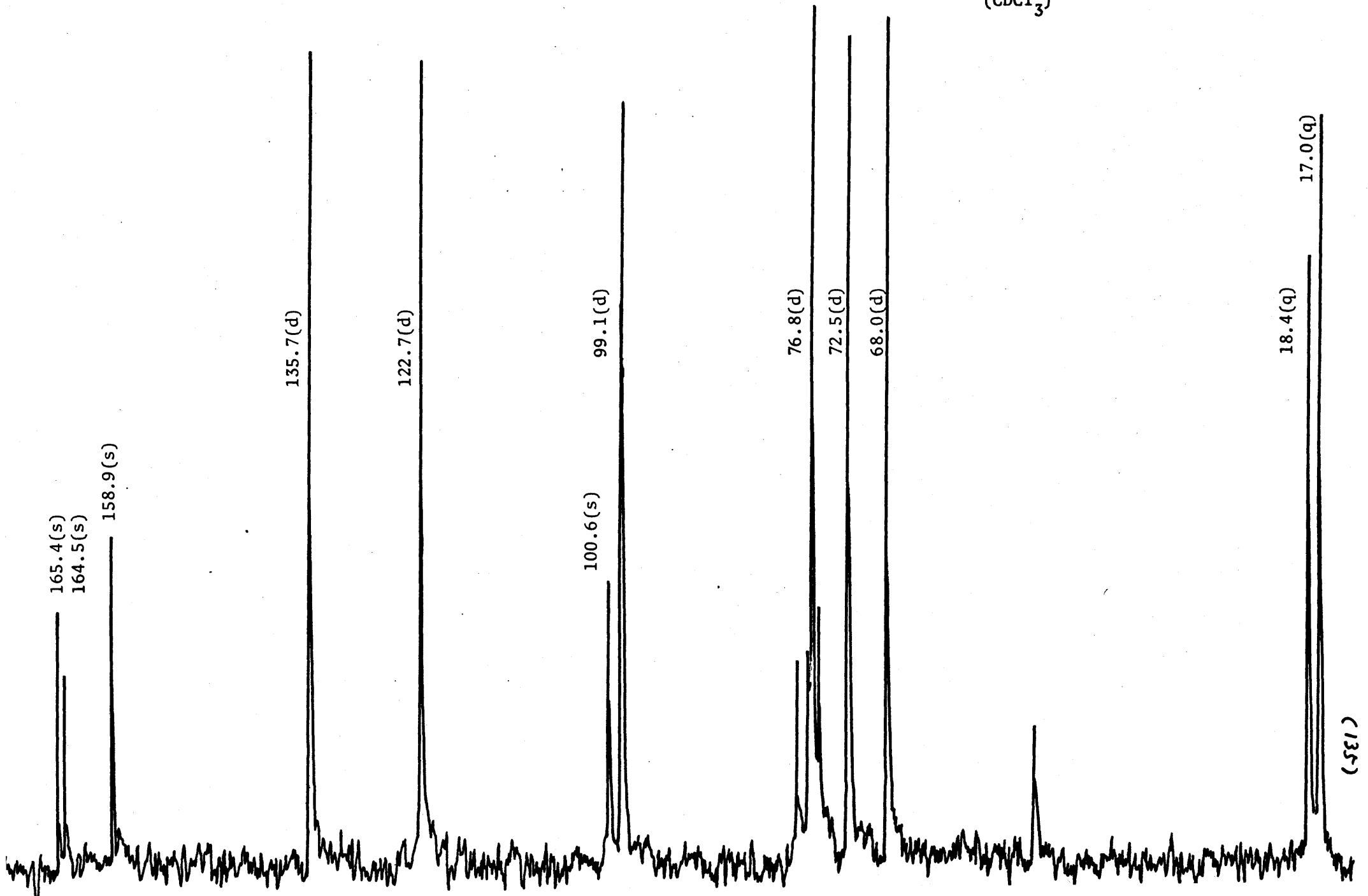
Fig. Proton Noise Decoupled C^{13} -NMR spectrum of radicicol.
