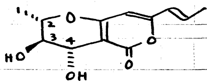
radicinol (2S, 3R, 4R)
