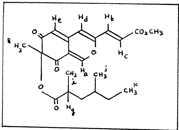
Fig. 2-5 Pmr spectrum of lunatoic acid A methyl ester. (CDCl 3 )
