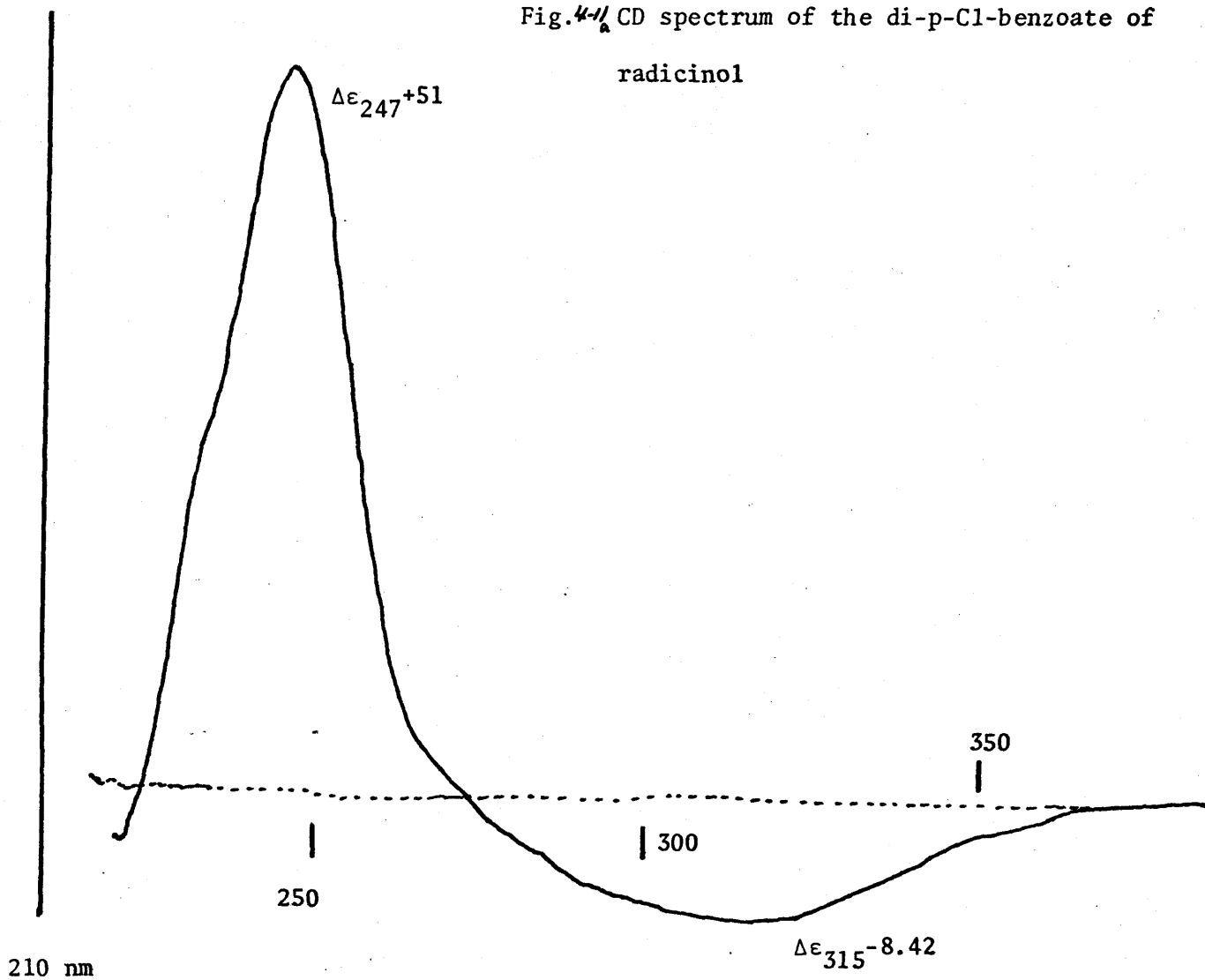
Fig. 4-11 b CD spectrum of the di-p-Cl-benzoate of 4-epi-radicalol
