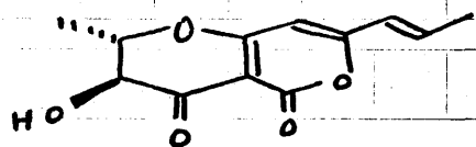
radicinin (2S, 3S)
