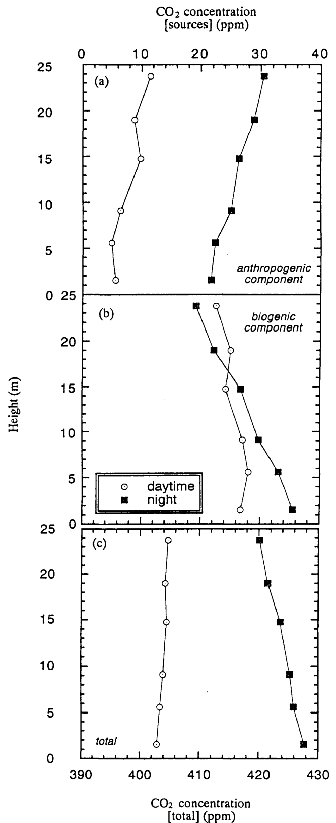
Fig. 7 The vertical profiles of mean concentration for anthropogenic (a), biogenic (b) and total CO 2 (c) components during the daytime (circle) and night (square).
