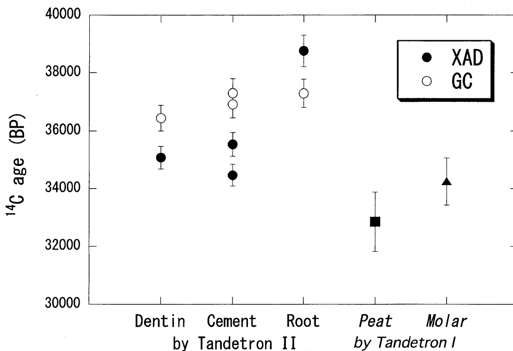
Fig. 5 ^{14}\text{C} ages of GC and XAD fractions for dentin, cement and root parts in the molar fossil of the Siberian Mammoth.
