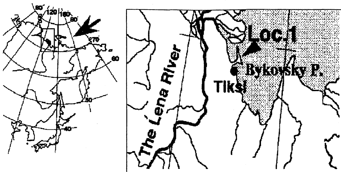
Fig. 1 Sampling point of a Mammoth molar fossil
