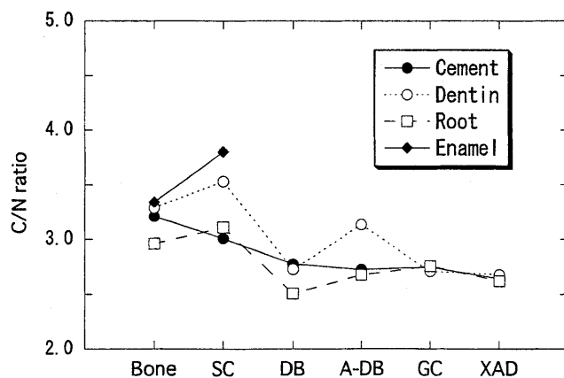
Fig. 3 C/N ratios of some fractions extracted from the molar fossil of the Siberian Mammoth.
