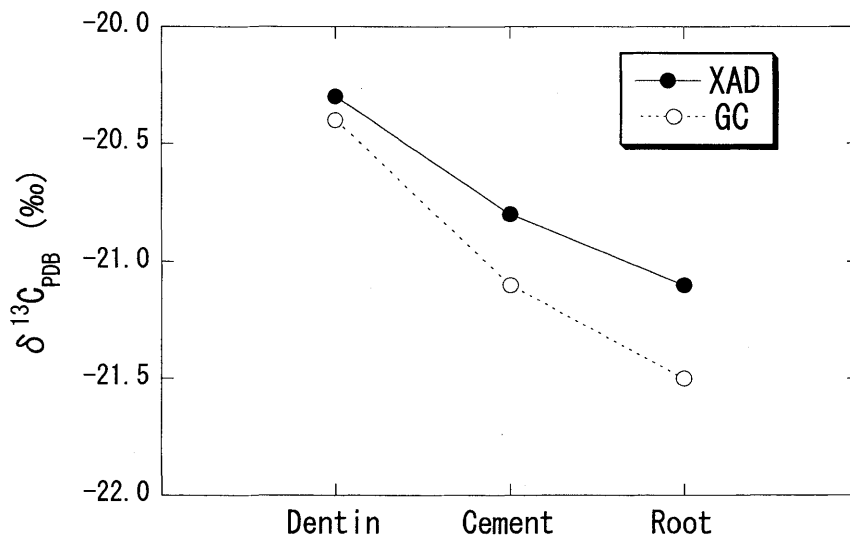
Fig. 4 \delta^{13}\text{C} values of GC and XAD fractions for dentin, cement and root parts in the molar fossil of the Siberian Mammoth.
