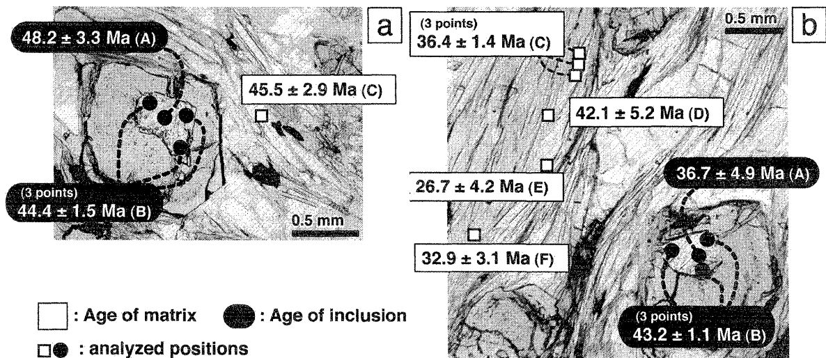
Fig. 4. Ar/Ar spot ages of phengites in the garnet-phengite schist from the Lago di Cignana area, Western Alps (after Gouzu et al., 2006a).
