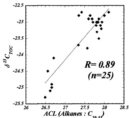
Fig. 7 Correlations between ACL and \delta^{13}C_{TOC} .
