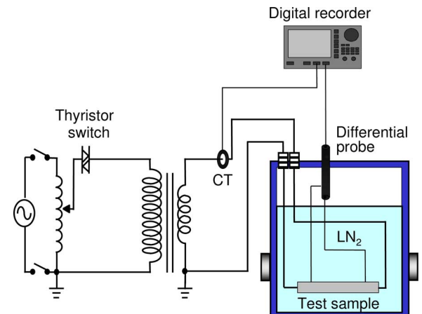
Fig. 3. Experimental setup.
