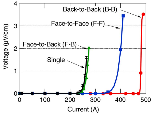
Fig. 4. Voltage-current characteristics of parallel-connected YBCO coated conductors.
