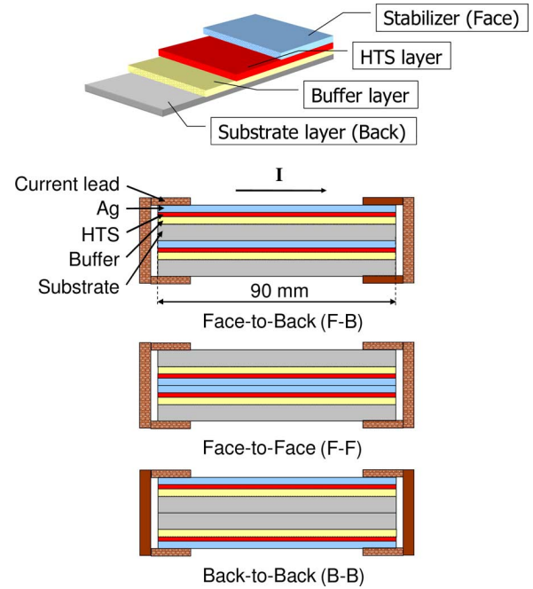
Fig. 2. Test samples.
