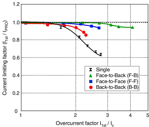
Fig. 8. Current limiting factor I_{1st}/I_{PRO} as a function of overcurrent factor I_{1st}/I_c .
