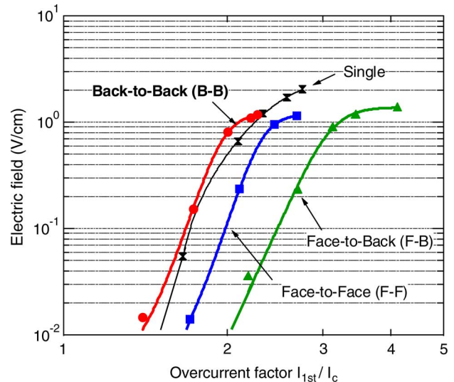
Fig. 7. Electric field as a function of overcurrent factor I_{1st}/I_C .
