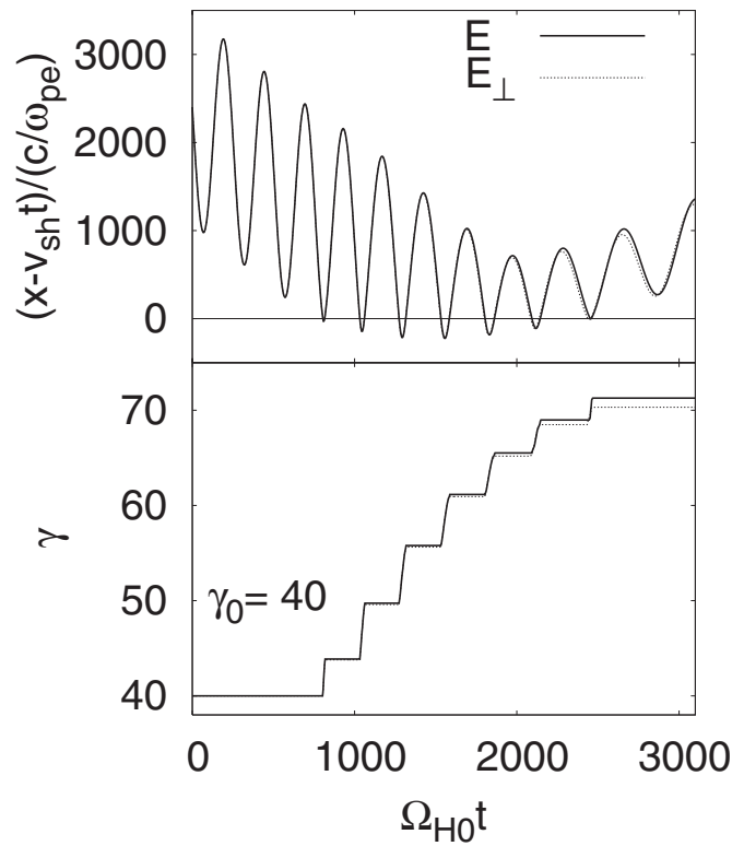
FIG. 3. Time variations in (x - v_{sh}t)/(c/\omega_{pe}) and \gamma . The solid and dotted lines, respectively, show the values calculated with use of E and with E_{\perp} . In the present case ( \gamma_0 = 40 ), the solid and dotted lines are quite close.
