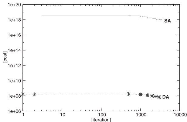
Fig. 5 Experimental result 2-1. (Change in the cost of DASA as a function of iteration counts of DA and SA. J_{m=1} for the DA stage and J_{m=1} + K \sum_{k=1}^n (\sum_{i=1}^c u_{ik} - 1)^2 for the SA stage against t_{DA} + t_{SA} .)
