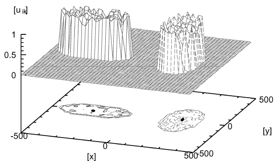
Fig. 6 Experimental result 3. (Fuzzy clustering result of elliptical distributions obtained using DASA. Data plotted on the xy plane show the cross sections of u_{ik} at 0.2 and 0.8. Black circles indicate centers of clusters.)
