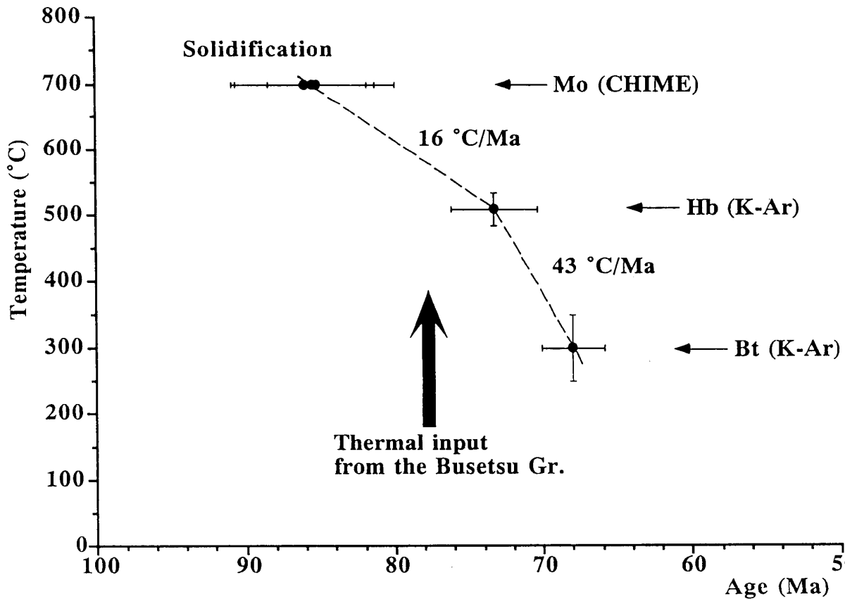
Fig. 4. Cooling history for the Shinshiro Tonalite from the solidification (700°C) to the closure temperature for biotite in K-Ar system (300°C). Average cooling rates are also shown. The emplacement age for the Busetsu Granite is based on its CHIME monazite ages (Suzuki et al., 1994b).
