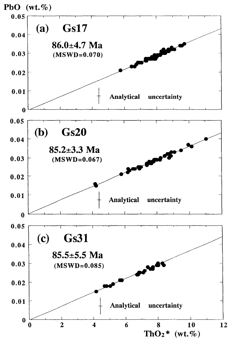
Fig. 2. \text{PbO-ThO}_2^* plots for monazite from sample Gs17 (a), sample Gs20 (b) and sample Gs31 (c). Error bars in the figures represent 2\sigma analytical uncertainty, and errors given to the ages are of 2\sigma .
