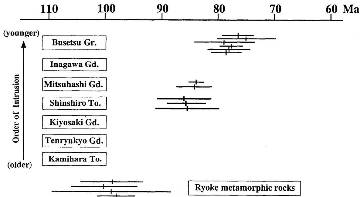
Fig. 3. Summary of CHIME monazite ages obtained in this study and those reported by Suzuki et al. (1994a,b). CHIME age data are in harmony with the order of intrusion.
