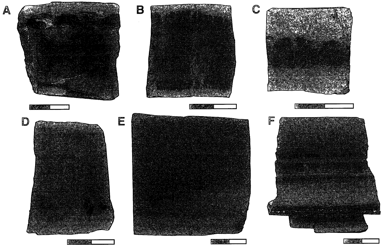
Fig. 4. Polished surfaces of black chert (A-D) and nectic chert (E and F) samples from the Anmenkou section. Sampling horizons are shown in Fig. 2. All scale bars indicate 2cm. A) CH-01. B) CH-24. C) CH-27. D) CH-39. E) NEC-01. F) NEC-03.
