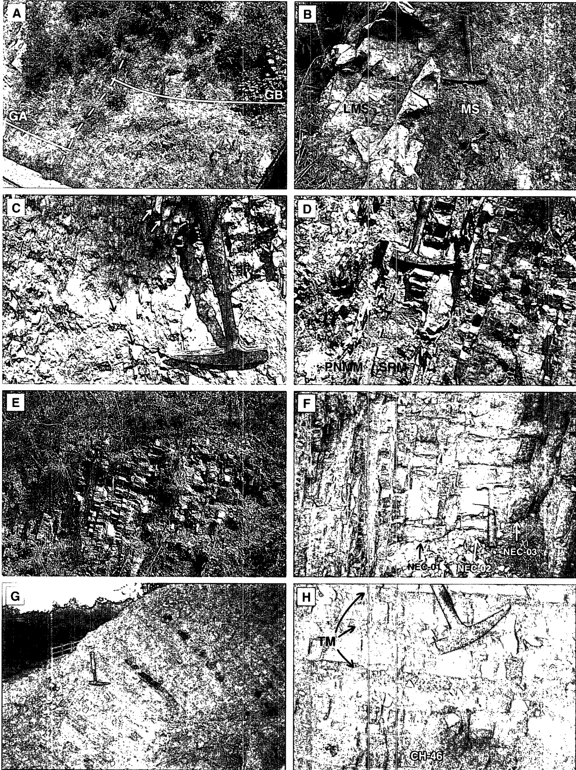
Fig. 3. Photographs of the outcrops in the Anmenkou section. A) An overall view of the GA and GB sections. Dotted line indicates the tuffaceous mudstone bed located in the top of the GA section and the base of the GB section. B) Disconformity between limestone of the Qixia Formation (LMS) and mudstone of the Gufeng Formation (MS). C) Phosphate nodules (arrows) included in mudstone of the Phosphate nodule-bearing mudstone Member. D) Boundary between the Phosphate nodule-bearing mudstone Member (PNMM) and Siliceous Rock Member (SRM). E) Upper part of the GA section consists of chert-rich alternating beds of chert and mudstone. F) Lower part of the GB section containing three intercalated netic chert beds. G) Middle part of the GD section consists of mudstone-rich alternating beds of chert and mudstone. Note that the beds are overturned. H) Alternating beds of chert, mudstone and tuffaceous mudstone (TM) around the sampling horizon of CH-46. Note that the beds are overturned.
