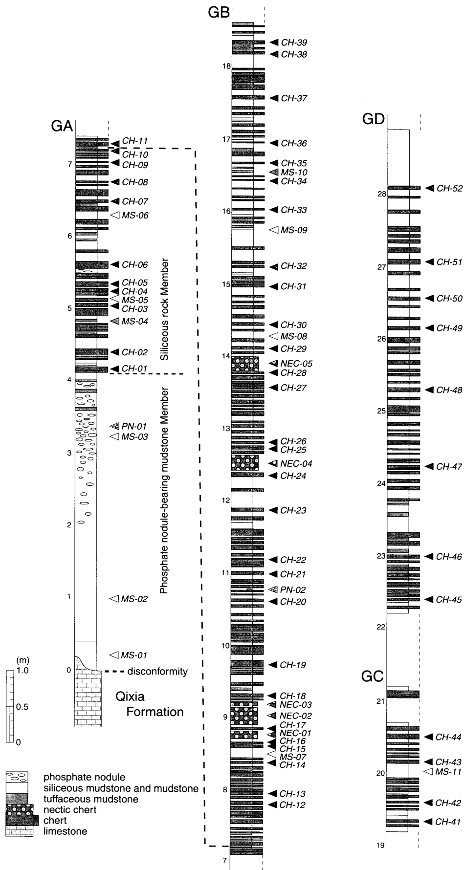
Fig. 2. Columnar section of the Gufeng Formation in the Anmenkou section.
