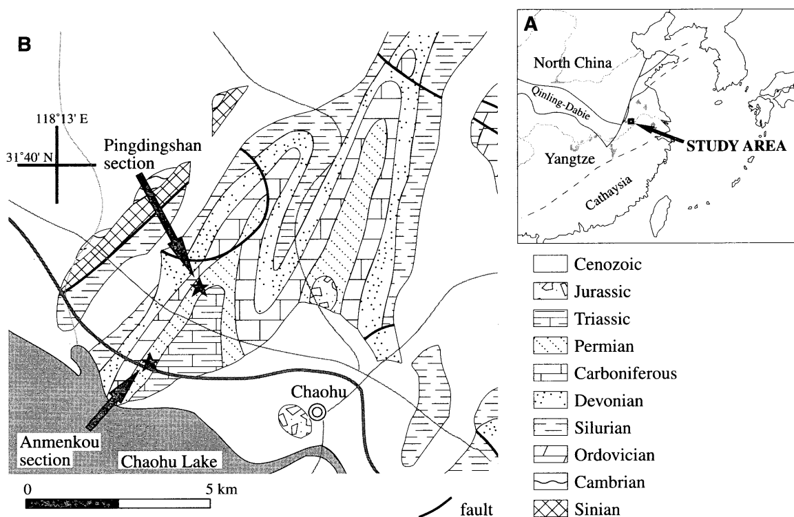
Fig. 1. A) Location map of the Chaohu area in the Yangtze Platform. B) Geological map of the Chaohu area (after Bureau of Geology and Mineral Resources of Anhui Province, 1987).
