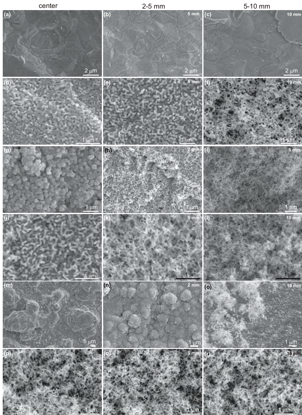
Figure 4: SEM micrographs of (a-c) W1 ( V_W = 13 V), (d-f) W2 ( V_W = 22 V), (g-i) W3 ( V_W = 34 V), (j-l) W4 ( V_W = 45 V), (m-o) W5 ( V_W = 55 V), and (p-r) W6 ( V_W = 62 V) at three different locations, i.e. at the center (leftmost), 2-5 mm (center), and 5-10 mm (rightmost).
