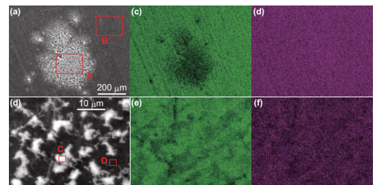
Figure 8: EDS mappings of sample W5 around fuzz region at r \sim 10 \text{ mm} with two areas ((a,b,c) and (d,e,f)) with different magnifications. (a,d) SEM images, (c,e) W signal profiles, and (d,f) Mo signal profiles. White region in (a,d) corresponds to fuzz areas.
