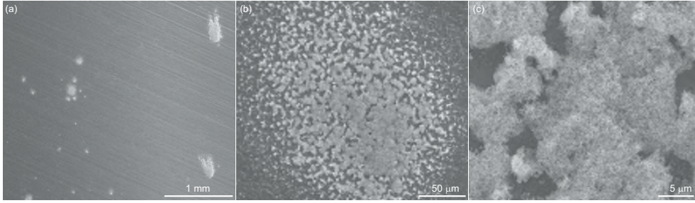
Figure 5: SEM micrographs of the peripheral region of W5 at different magnifications. In (b), one of the white areas in (a) is shown in a larger magnification. In the white areas, FNAs are grown locally, as shown in (c).
