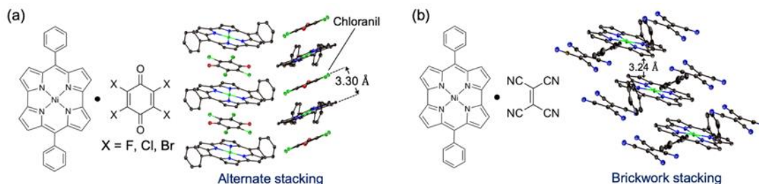
Figure 4. X-ray structure of (a) Ni(II) meso -diphenylnorcorrole and benzoquinones (b) Ni(II) meso -diphenylnorcorrole and TCNE co-crystals.
