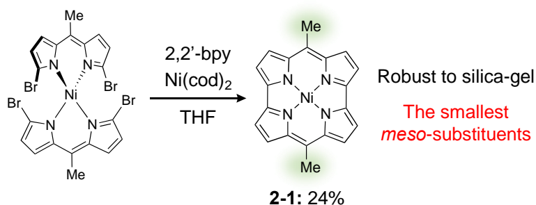
Scheme 1. Synthesis of Ni(II) meso -dimethylnorcorrole 2-1 .
