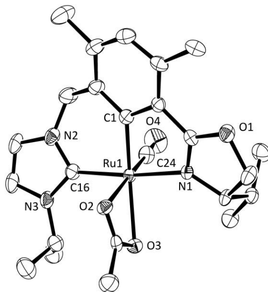
Figure 4. ORTEP diagram of 9b at the 50% probability level. Selected bond lengths (Å) and angles (°): Ru1-C1 2.010(3), Ru1-C16 2.039(3), Ru1-C24 1.784(3), Ru1-N1 2.121(2), Ru1-O2 2.1956(19), Ru1-O3 2.310(2), O4-C24 1.172(4).
