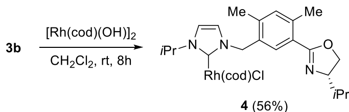
Scheme 2. Preparation of NHC Rh complex.
