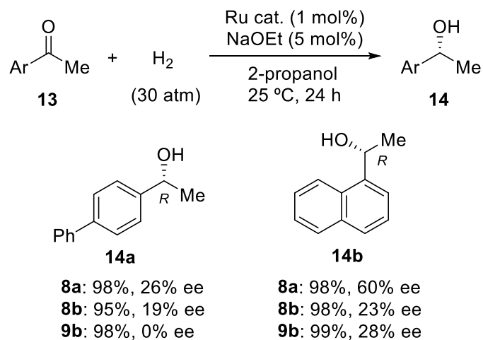
Scheme 6. Hydrogenation of ketones catalyzed by 8a–b .
