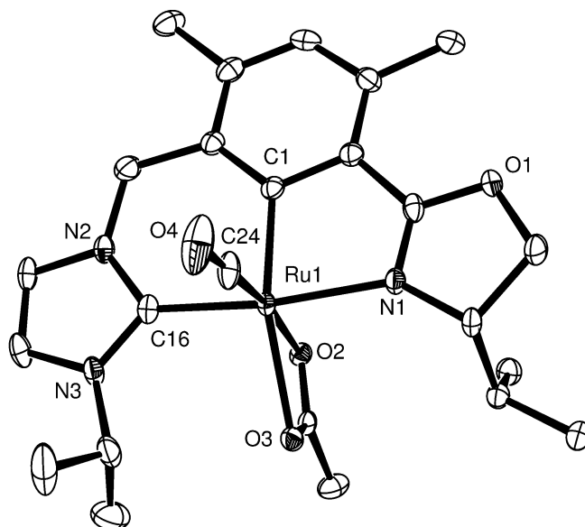
Figure 3. ORTEP diagram of 8b at the 50% probability level. Selected bond lengths (Å) and angles (°): Ru1-C1 2.020(3), Ru1-C16 2.013(4), Ru1-C24 1.798(4), Ru1-N1 2.155(3), Ru1-O2 2.211(2), Ru1-O3 2.277(2), O4-C24 1.167(5); C16-Ru1-N1 171.69(12), C1-Ru1-O3 153.62(11), C1-Ru1-O2 96.30(10), C24-Ru1-C1 89.58(15), C24-Ru1-O2 173.34(14), O4-C24-Ru1 175.4(4), N2-C16-Ru1 127.0(3), N3-C16-Ru1 129.7(3), N2-C16-N3 103.2(3).
