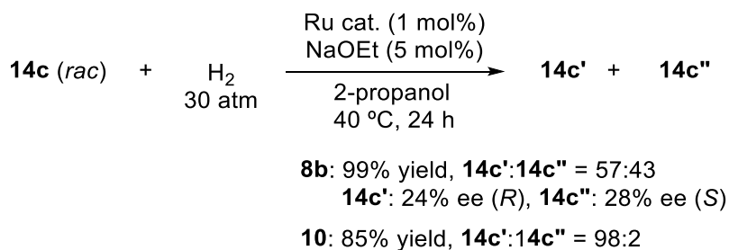
Scheme 7. Hydrogenation of 14c catalyzed by 8b and 10 .
