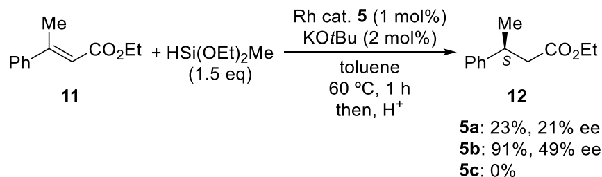
Scheme 5. Asymmetric conjugate reduction of 11 .
