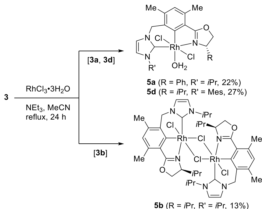
Scheme 3. Preparation of CCN pincer Rh complexes.
