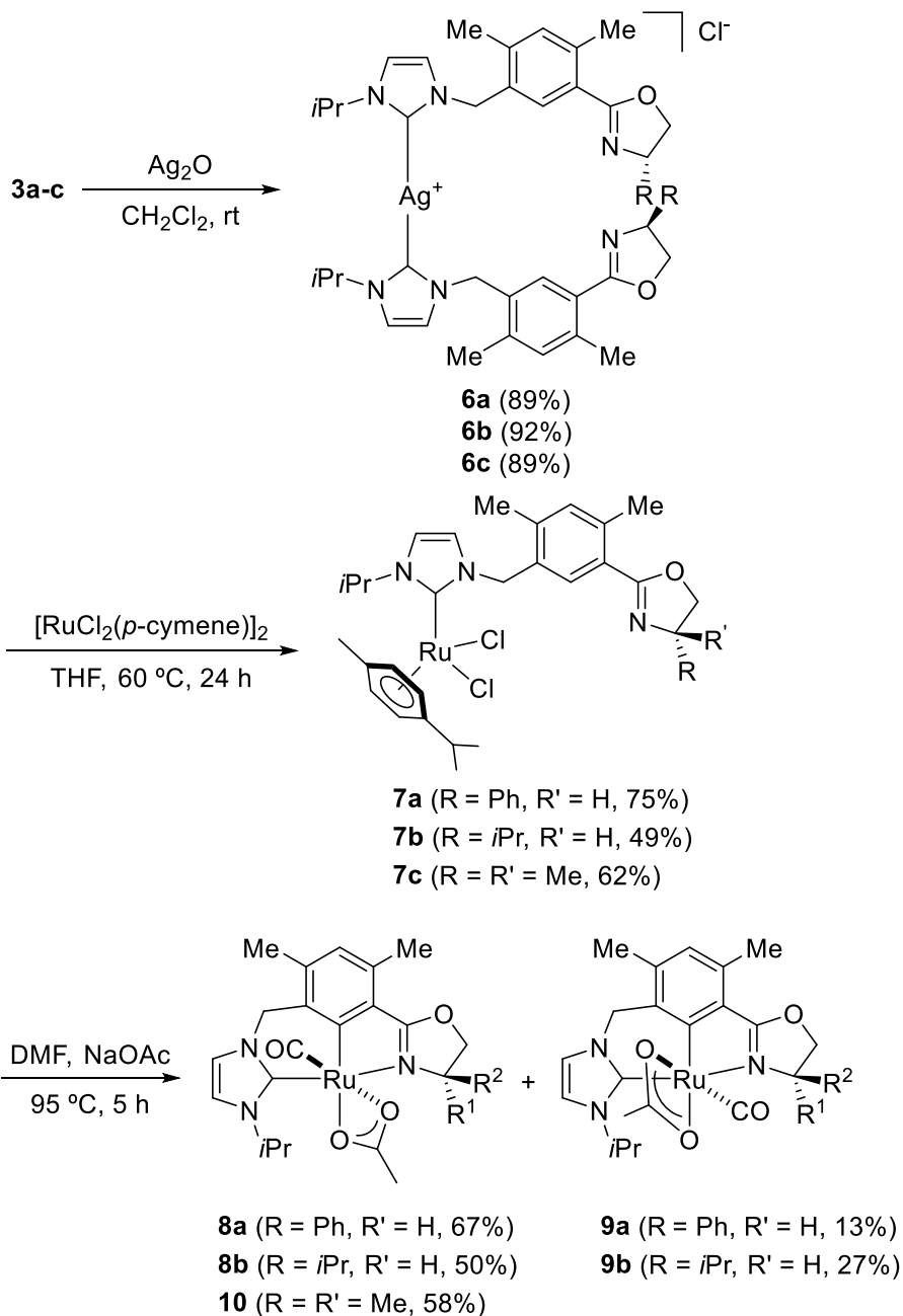
Scheme 4. Preparation of CCN pincer Ru complexes.
