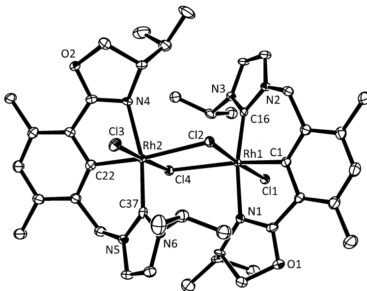
Figure 1. ORTEP diagram of 5b at the 50% probability level. Selected bond lengths (Å) and angles (°): Rh1-C1 1.979(4), Rh1-C16 1.975(4), Rh1-N1 2.097(3), Rh1-C11 2.3284(10), Rh1-Cl2 2.3716(10), Rh1-Cl4 2.6131(10), Rh2-C22 1.988(4), Rh2-C37 1.976(4), Rh2-N4 2.143(3), Rh2-Cl2 2.5275(9), Rh2-Cl3 2.3347(10), Rh2-Cl4 2.3760(10), C16-Rh1-N1 169.38(15), C11-Rh1-Cl2 176.82(3), C1-Rh1-Cl4 164.57(11), C37-Rh2-N4 166.19(14), Cl3-Rh2-Cl4 177.90(4), C22-Rh2-Cl2 170.98(11), Rh1-Cl2-Rh2 98.29(3), Rh2-Cl4-Rh1 95.86(3).
