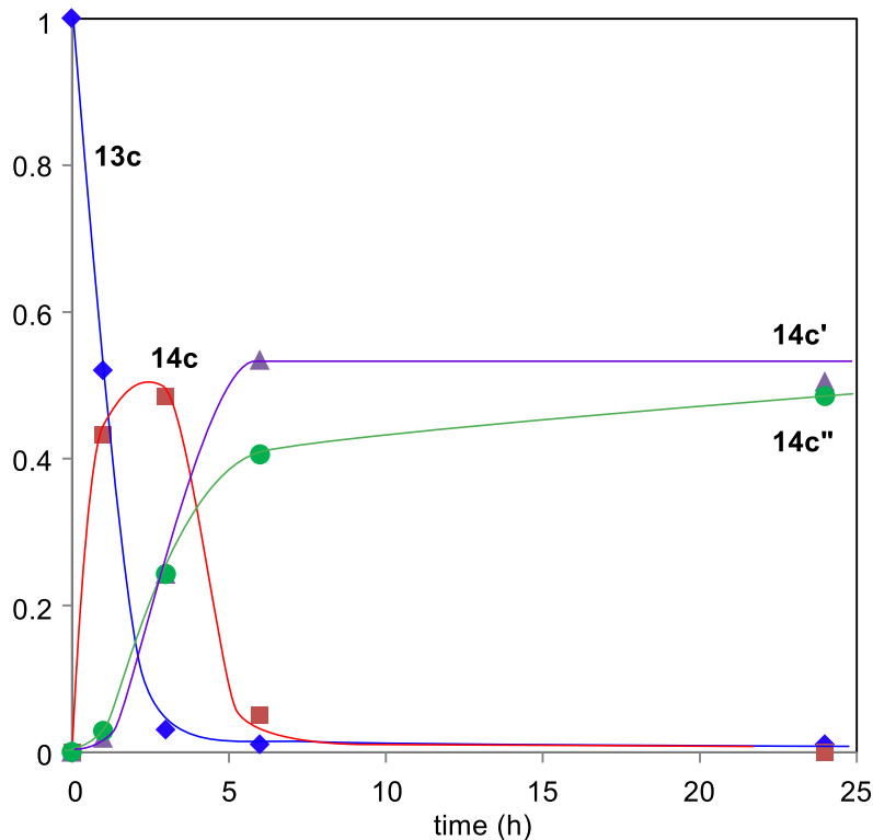
Figure 5. Time conversion of hydrogenation (30 atm) of 13c catalyzed by 8b (1 mol%) and NaOEt (5 mol%) in 2-propanol at 40°C.
