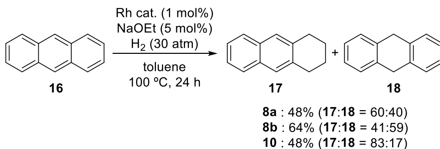
Scheme 8. Hydrogenation of 16 catalyzed by 8a,b and 10 .
