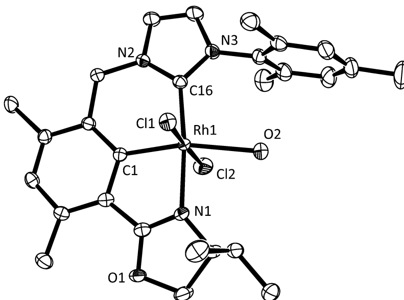
Figure 1. ORTEP diagram of 5b at the 50% probability level. Selected bond lengths (Å) and angles (°): Rh1-C1 1.979(4), Rh1-C16 1.975(4), Rh1-N1 2.097(3), Rh1-C11 2.3284(10), Rh1-Cl2 2.3716(10), Rh1-Cl4 2.6131(10), Rh2-C22 1.988(4), Rh2-C37 1.976(4), Rh2-N4 2.143(3), Rh2-Cl2 2.5275(9), Rh2-Cl3 2.3347(10), Rh2-Cl4 2.3760(10), C16-Rh1-N1 169.38(15), C11-Rh1-Cl2 176.82(3), C1-Rh1-Cl4 164.57(11), C37-Rh2-N4 166.19(14), Cl3-Rh2-Cl4 177.90(4), C22-Rh2-Cl2 170.98(11), Rh1-Cl2-Rh2 98.29(3), Rh2-Cl4-Rh1 95.86(3).
