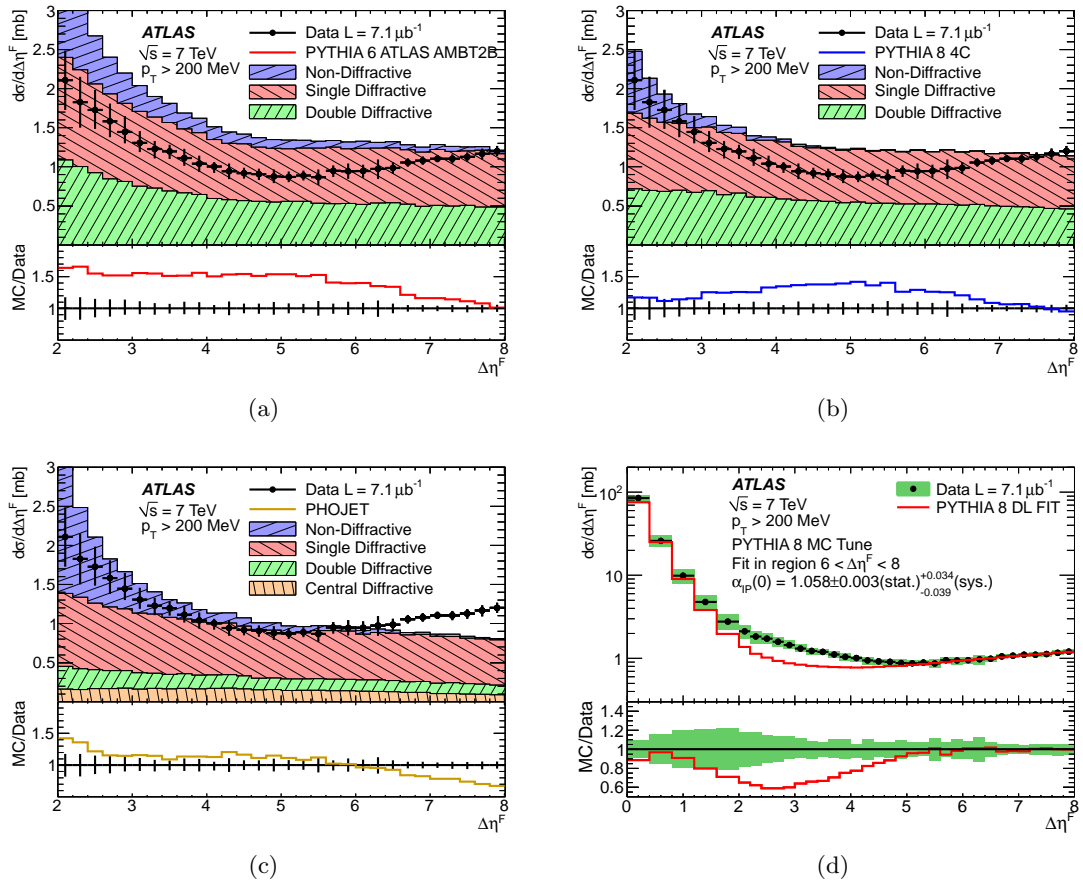
FIGURE 2.3: Cross-section of rapidity gap measured with the ATLAS detector in p - p collisions at \sqrt{s}=7 TeV. Inelastic differential cross-section shown as a function of forward gap size \Delta\eta^F for particles with p_T > 200 MeV. The hatched area indicates the total uncertainties. The full lines represent the MC simulations by using PHOJET and the default versions of PYTHIA6 and PYTHIA8. The dashed lines show the different contributions of the SD, DD and ND processes according to the models [50].
