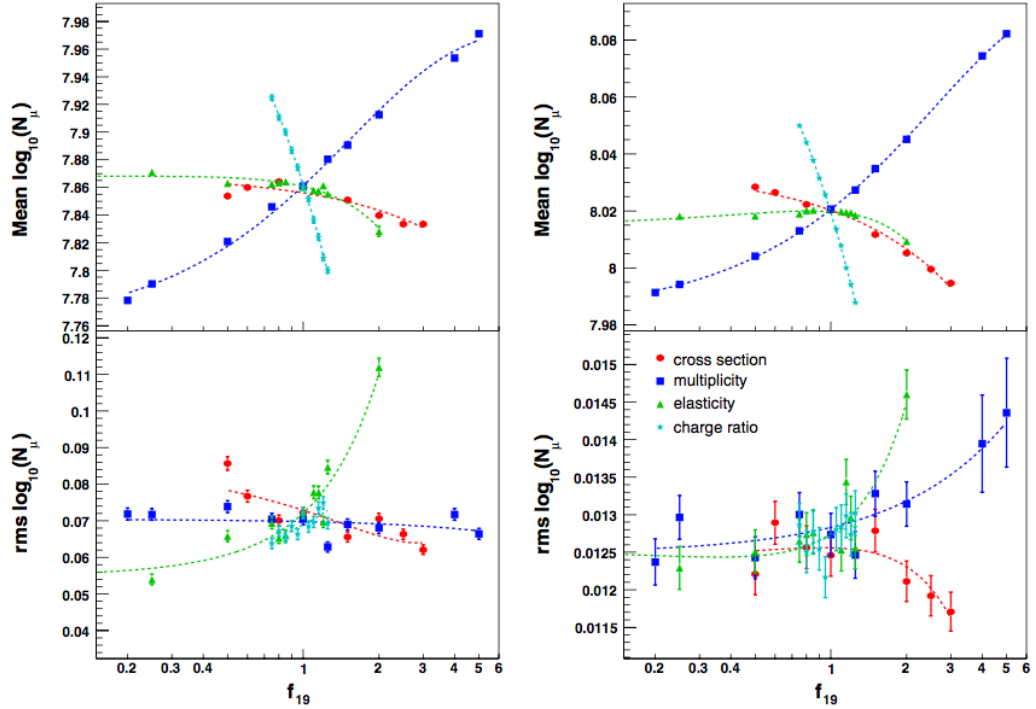
FIGURE 1.9: The mean (top) and the standard deviation (bottom) of \log_{10}(N_\mu) predicted by SIBYLL2.1, corresponding to 10^{19.5} eV proton (left) and iron (right) primaries [19]. Different color lines and markers indicate the effect of each parameter to the determination of \log_{10}(N_\mu) and \sigma \log_{10}(N_\mu) based on an artificial shift in single corresponding parameter [19].
