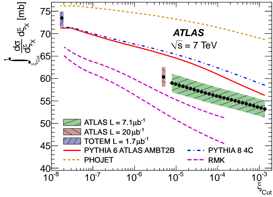
FIGURE 2.4: Inelastic cross-section shown as a function of \xi_X < \xi_{Cut} . It is calculated by integrating the differential cross-section from rapidity gap sizes of zero to a certain variable, excluding the diffractive dissociation with \xi_X < \xi_{Cut} . The results are carried out by using the data measured by ATLAS detector at \sqrt{s} = 7 TeV (ATLAS L = 7.1 \mu b^{-1} ). TOTEM results and ATLAS results from different data set are shown as references at different integration ranges.[50].
