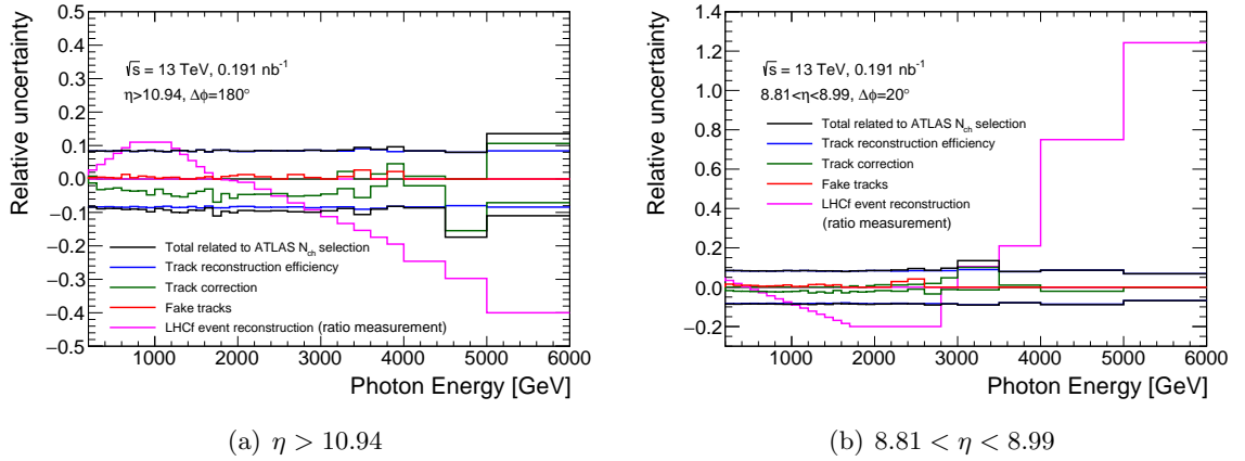
FIGURE 5.16: Summary of systematic uncertainties related with ATLAS event selection. The uncertainties are assigned to the N_\gamma^{N_{\text{ch}}=0} spectra and to the N_\gamma^{N_{\text{ch}}=0}/N_\gamma^{\text{all}} ratio. Additionally, the systematic uncertainty on the ratio related with LHCf photon selection is shown as a reference.
