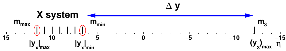
FIGURE 2.2: Pseudo-rapidity distribution image of single diffractive dissociation. The X system consists of many secondary particles produced by the incident particle.
