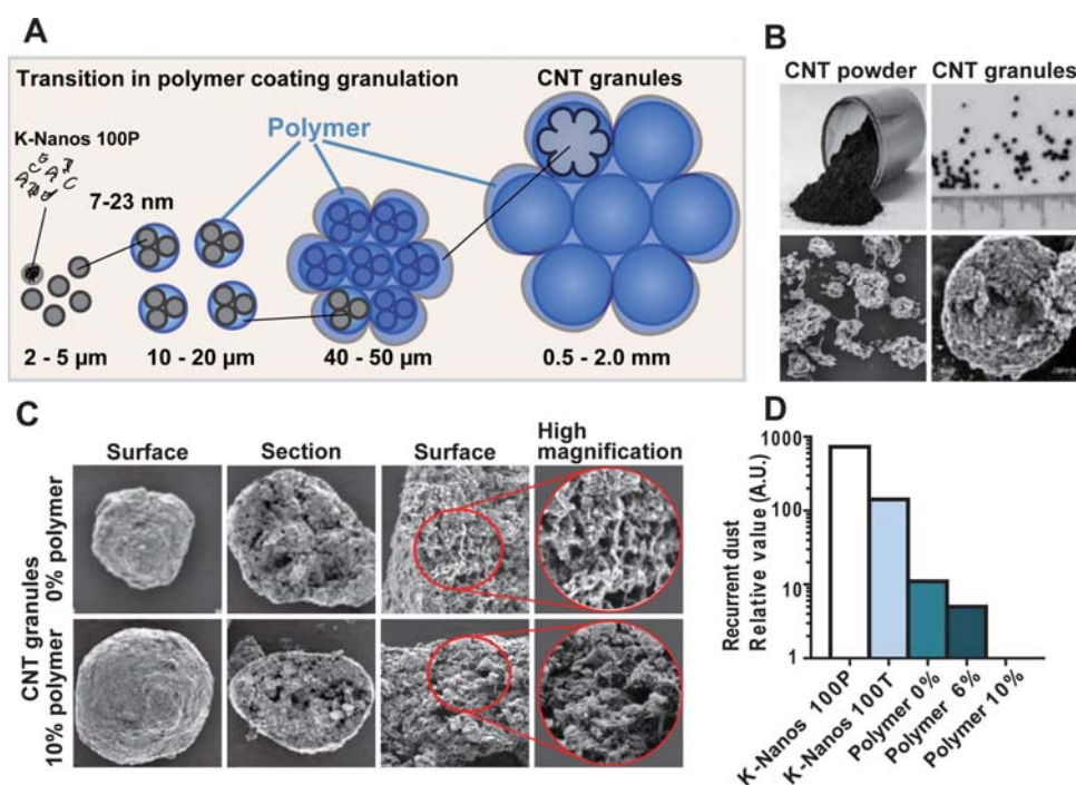
Fig. 1 Carbon nanotube (CNT) granules generated by polymer coating reduce the dustability (A) Procedure to generate CNT granules with polymer coating. (B) Metamorphosis of K-nanos 100P from CNT powder to granules. Lower panels, scanning electron microscopy (SEM). (C) SEM images in CNT granules with or without polymer coating. (D) Dustability of each CNT evaluated by recurrent dust.
