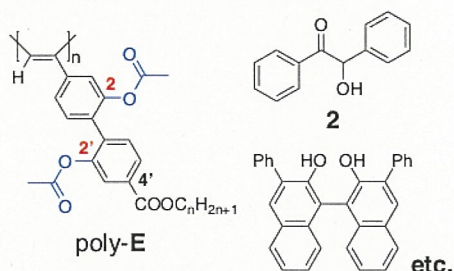
Figure 3. Structures of poly-E and racemates.
