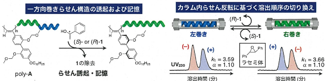
Figure 1. Schematic illustration of the helicity induction and memory of poly-A and a poly-A-based CSP capable of switching the elution order of enantiomers in HPLC.
