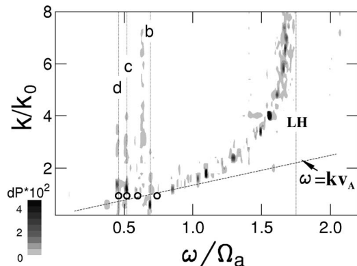
FIG. 8. An increase in P , dP(k, \omega) = P_2(k, \omega) - P_1(k, \omega) , in the four-ion-species plasma. The four vertical lines represent the lower hybrid resonance and heavy-ion cutoff frequencies.
