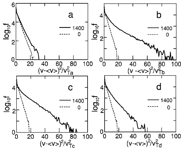
FIG. 10. Energy distribution functions of ions, f[(v - \langle v \rangle)^2] , at \Omega_a t = 0 and 1400. Here, v_{Ti} ( i = a, b, c, or d ) is the initial thermal velocity.
