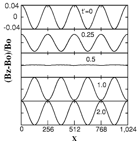
FIG. 1. Profiles of B_z in the single-ion-species plasma at times t' \approx k_0v_A t/\pi=0, 0.25, 0.5, 1.0, and 2.0 .
