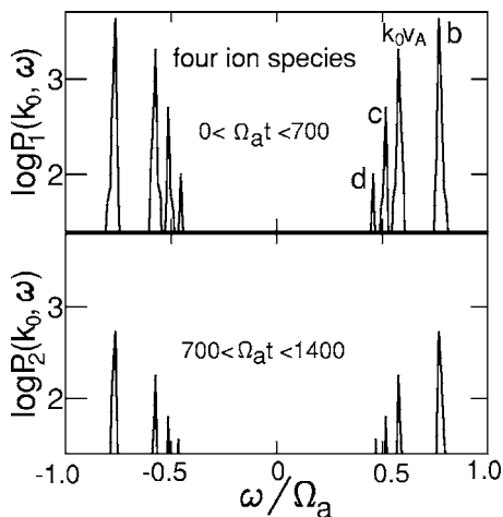
FIG. 7. The power spectra of magnetic fields with k=k_0 in the four-ion-species plasma. The heavy-ion cutoff frequencies are \omega_{b0}/\Omega_a=0.69 , \omega_{c0}/\Omega_a=0.52 , and \omega_{d0}/\Omega_a=0.46 , while the frequency of the magnetosonic mode is k_0 v_A/\Omega_a=0.60 .
