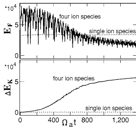
FIG. 9. Time variations of ion kinetic energies, E_F and E_K . The dashed and solid lines represent the energies in the single- and four-ion-species plasmas, respectively. The energy E_F of the single-ion-species plasma is averaged over the period k_0 v_A t = 2\pi .
