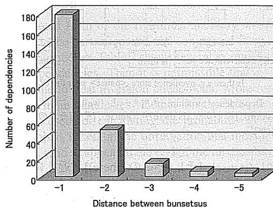
Fig. 9 Distance between bunsetsus of inversion.
