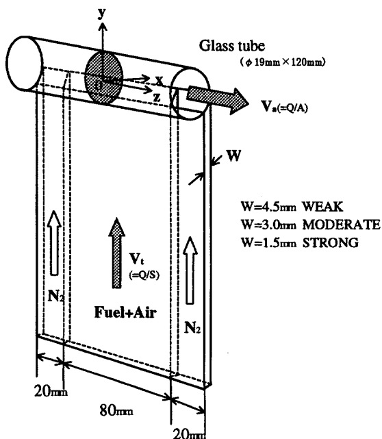
Fig. 1 Swirl-type burner
