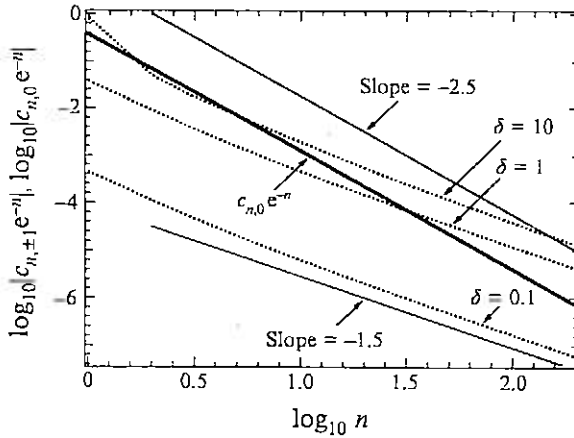
FIGURE 3. A plot of \log_{10}|c_{n,\pm 1}e^{-n}| vs. \log_{10}n by the numerical solutions of (4.14a) for the aspect ratio \delta = 0.1, 1 and 10 (broken lines). The values of \log_{10}|c_{n,0}e^{-n}| are also plotted (solid line). The thin straight lines have the indicated slopes.
